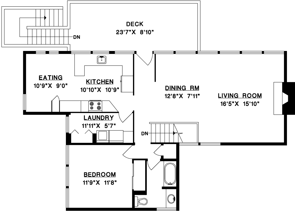
MAIN FLOOR
