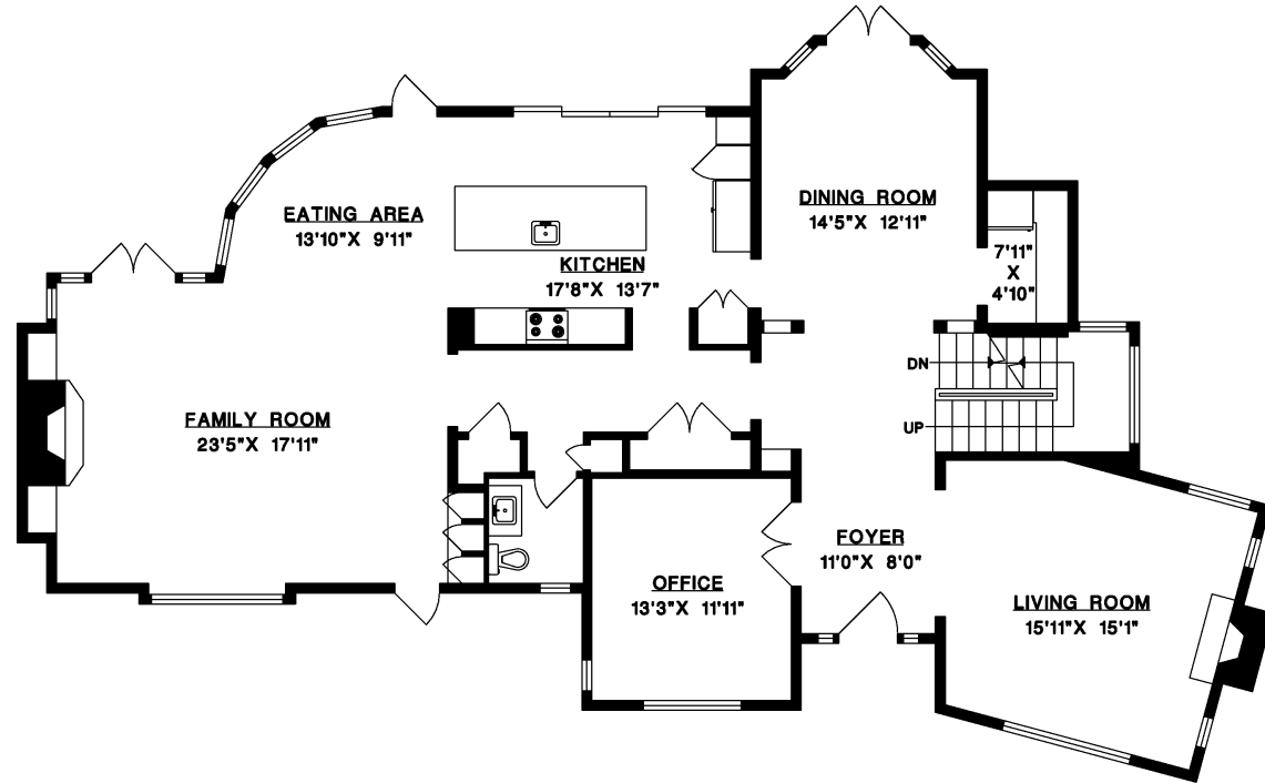
MAIN FLOOR
